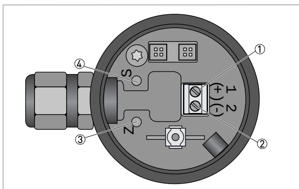
Figure 4-3: Connection in the terminal compartment
