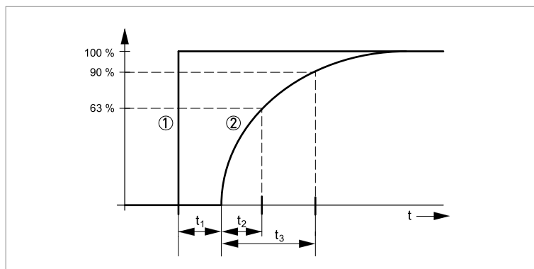
Figure 2-18: Behaviour at an abrupt change in the process variable. t_1 - dead time; t_2 - rise time t_{63} ; t_3 - rise time t_{90}
