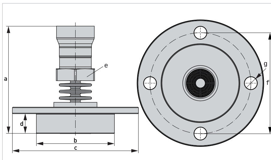
Figure 2-7: DRD flange
